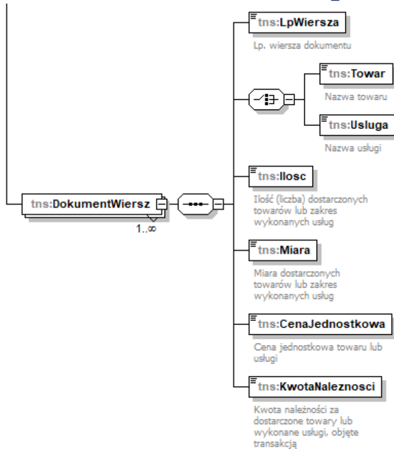
Diagram 7. The structure of the element DokumentWiersz of JPK_GV
