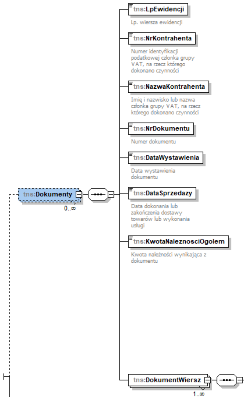
Diagram 6. The structure of the element Dokumenty of JPK_GV
