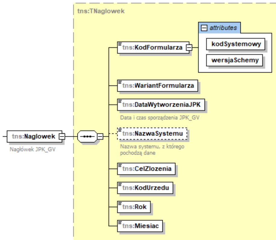
Diagram 2. The structure of the element Naglowek of JPK_GV
